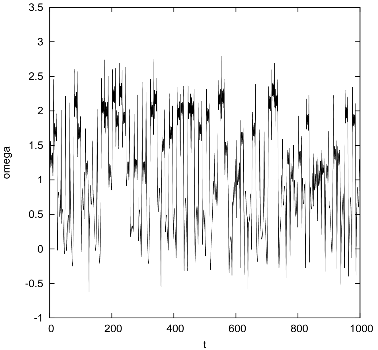
Orbiting Dumbbell Problem Elliptical Orbit -- Tolerance=10(-12)
